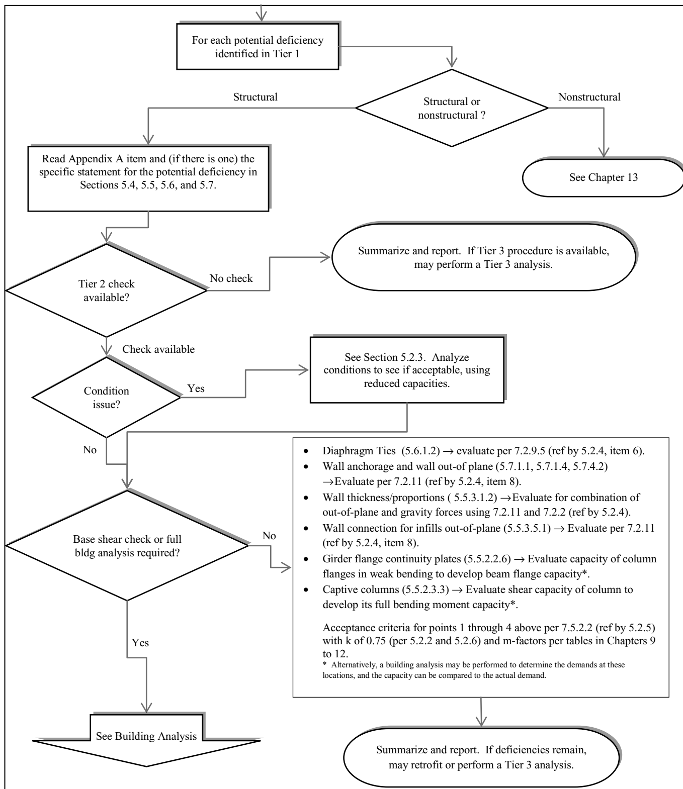
FIG. 5-1. Tier 2 Evaluation Process
