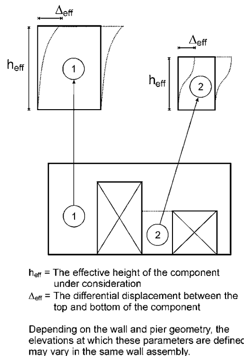
FIG. C11-1. Effective Height and Differential Displacement of Wall Components
