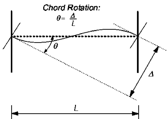
FIG. 10-6. Chord Rotation for Shear Wall Coupling Beams
