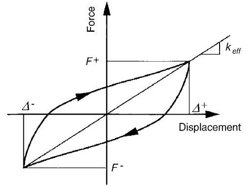
Hysteretic behavior
