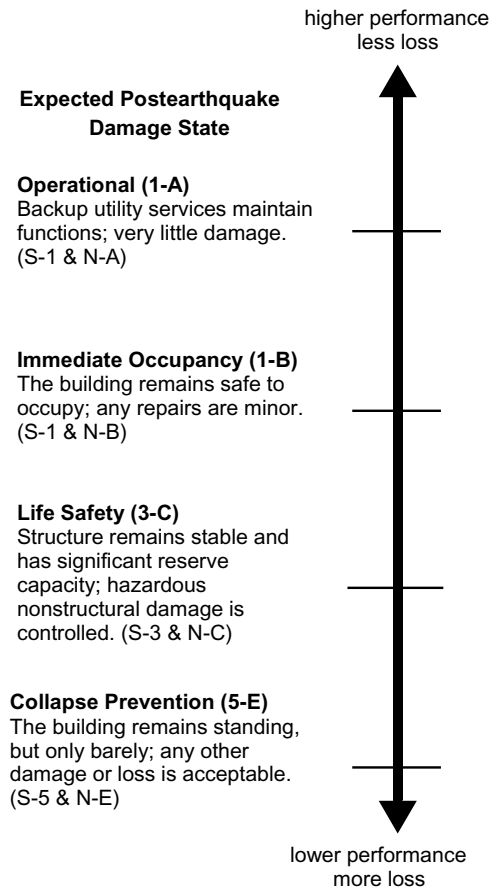
FIG. C2-1. Target Building Performance Levels and Ranges
