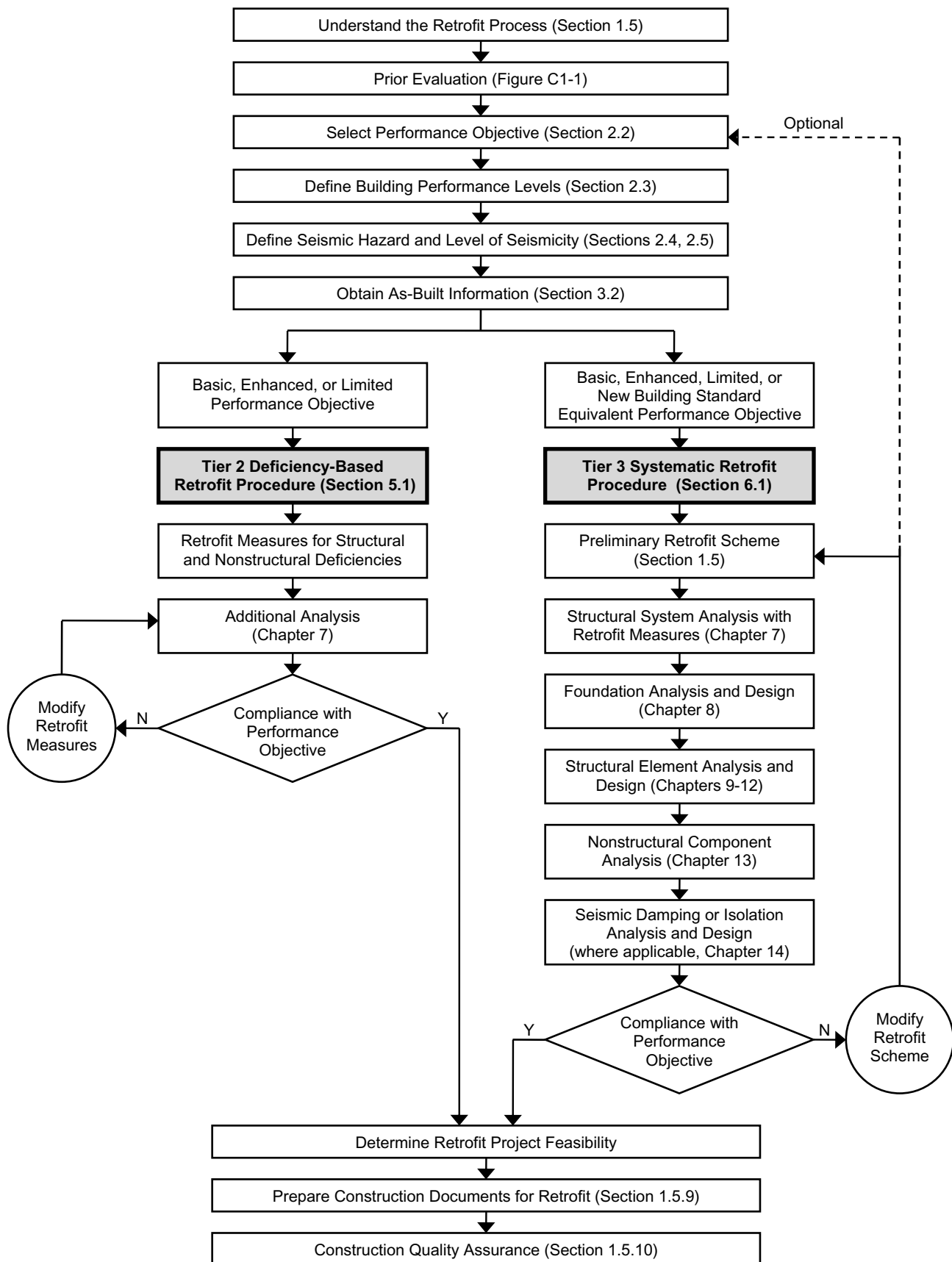
FIG. C1-2. Retrofit Process
