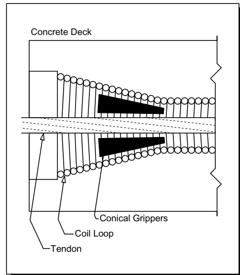
FIG. A-11. Coil Anchor
