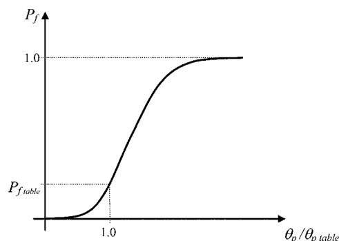
FIG. C10-1. Fragility Curve
